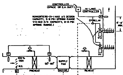
Fig. 16-5 SINGLE ZONE H.V. UNIT WITH INTERNAL F. AND B. DAMPERS - PRIMARY HUMIDIFICATION
