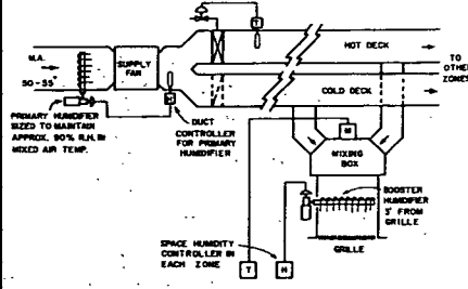
Fig. 16-6 HIGH VELOCITY, DUAL DUCT SYSTEM WITH PRIMARY AND BOOSTER HUMIDIFICATION
