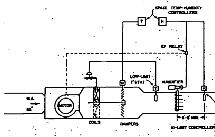
Fig. 16-5 SINGLE ZONE H.V. UNIT WITH INTERNAL F. AND B. DAMPERS - PRIMARY HUMIDIFICATION
