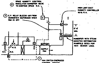
Fig. 16-3 100% OSA HEAT-VENT SYSTEM WITH SEQUENCE CONTROL ON PRIMARY HUMIDIFICATION
