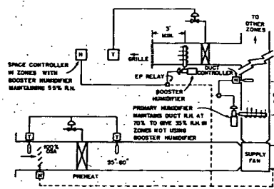
Fig. 16-4 100% OSA HEAT-VENT SYSTEM WITH PRIMARY HUMIDIFICATION
