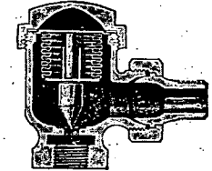
Sectional View
