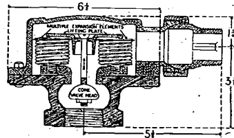
Section of 1 1/4" and 1 1/2" No. 9-3
