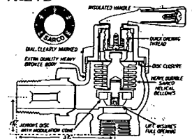
Section of 1/2" and 3/4" Valve
