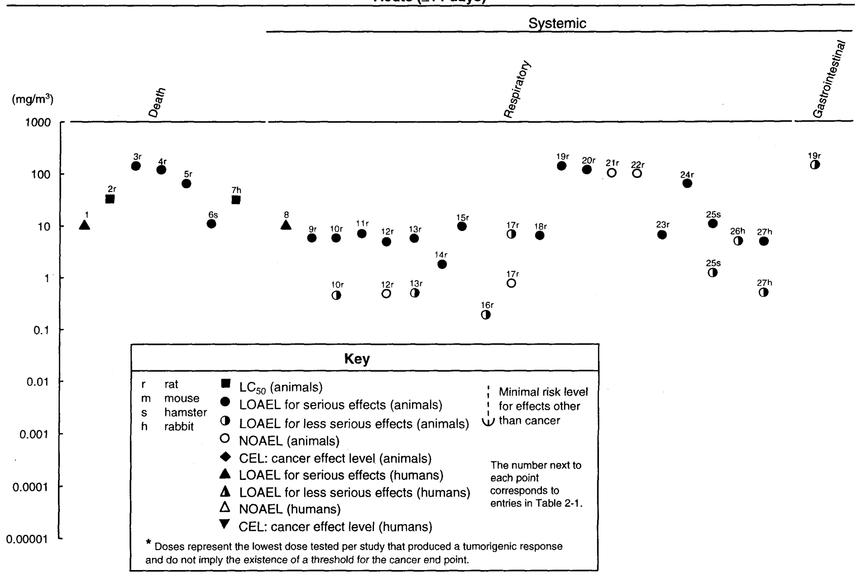
Figure 2-1. Levels of Significant Exposure to Cadmium - Inhalation Acute ( \leq 14 days)
