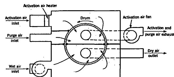
FIG. 4. SOLID ADSORBENT DEHYDRATOR—ROTATING BED TYPE
