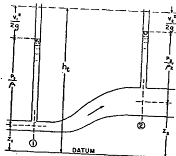
FIG. 1. RELATION OF VARIOUS FACTORS IN BERNOULLI EQUATION
