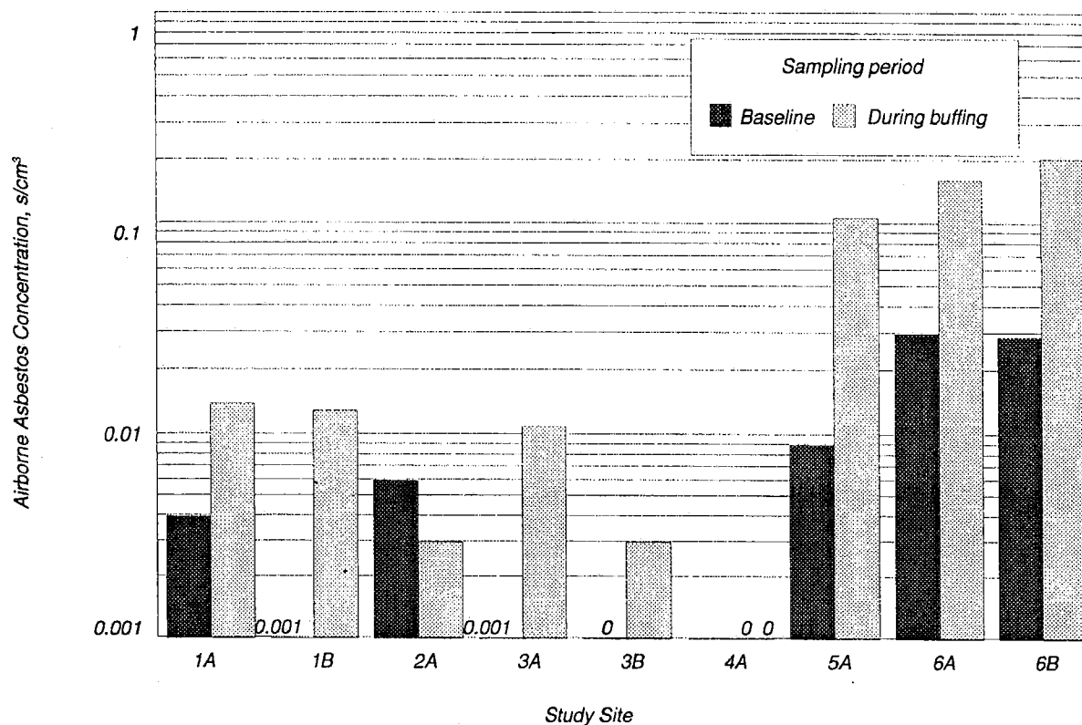
Figure 1. Average airborne asbestos concentrations (measured by TEM) before and during buffing of asbestos-containing resilient floor tile (continued).
