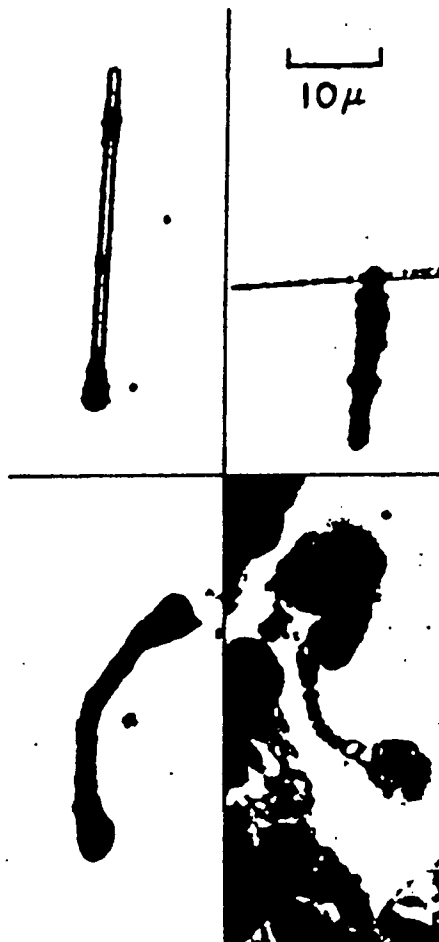
Fig 4.—Ferruginous bodies formed in response to other filamentous dusts and stained for iron (Peris' test). The central fiber (top, left and right) is silicon carbide; and (bottom left) tremolite (talc) ( \times 1,110 ).
