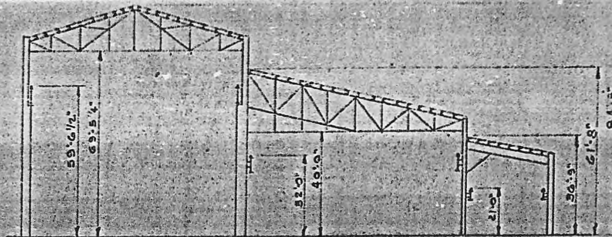
SECTION "A-A"
