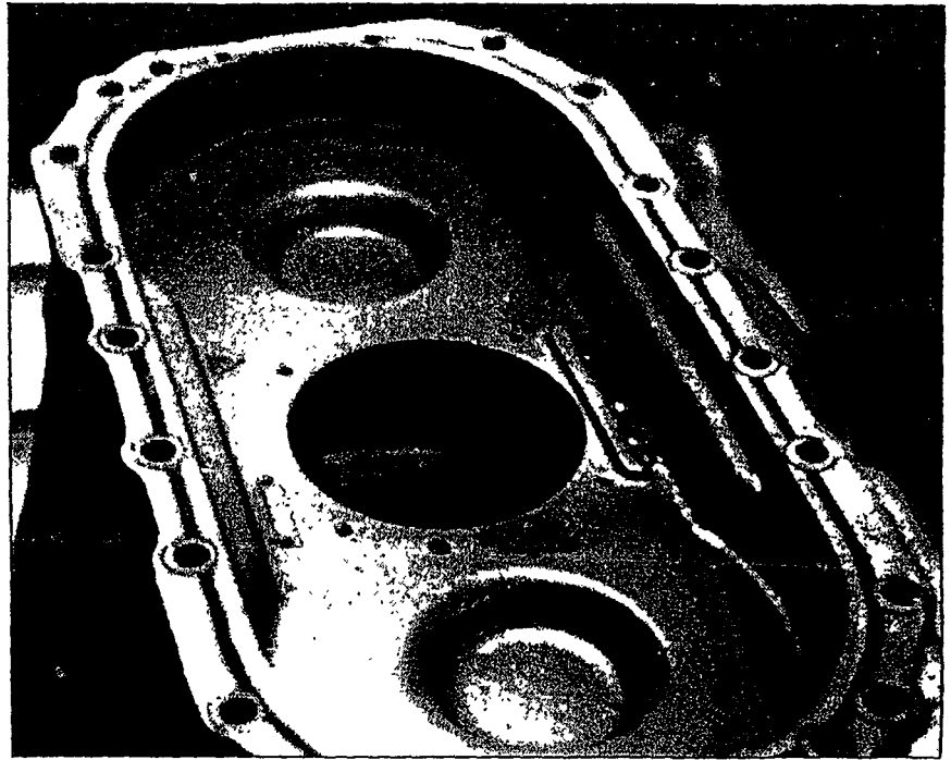
Anaerobic and other liquid sealants are one way to solve the problem of eliminating asbestos from many sealing products. Shown here is a 28 in. long housing with a liquid gasket seal ready for assembly.
