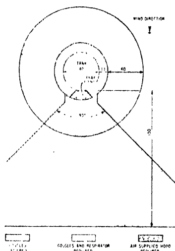
Figure 6. Personal protective devices as a function of areas around the structure being sprayed, wind direction, and spray point
