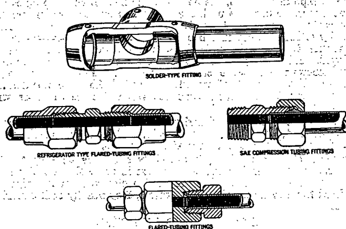
FIG. 2. COPPER OR BRASS TUBING FITTINGS
