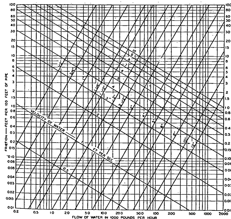
FIG. 23. FRICTION LOSS FOR 300 F WATER IN COMMERCIAL STEEL PIPE (SCHEDULE 40)
