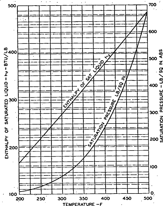
FIG. 22. RELATION OF SATURATION PRESSURE AND ENTHALPY TO WATER TEMPERATURE
