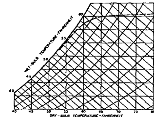
Fig. 12 . . . Performance of Dehumidifying Coil
