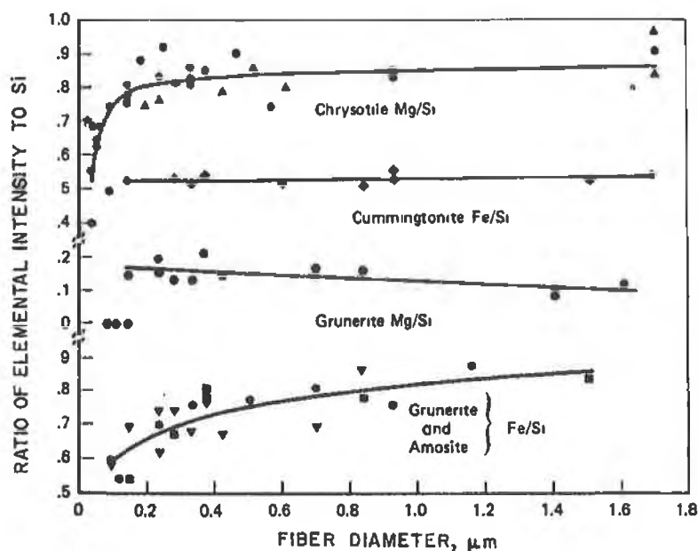
FIGURE 34. - Intensity ratio of FeK \alpha , MgK \alpha , or CaK \alpha relative to SiK \alpha as a function of fiber diameter. (Reprinted with permission of D. R. Beaman and D. M. File from Analytical Chemistry (2). Copyright by the American Chemical Society.)
