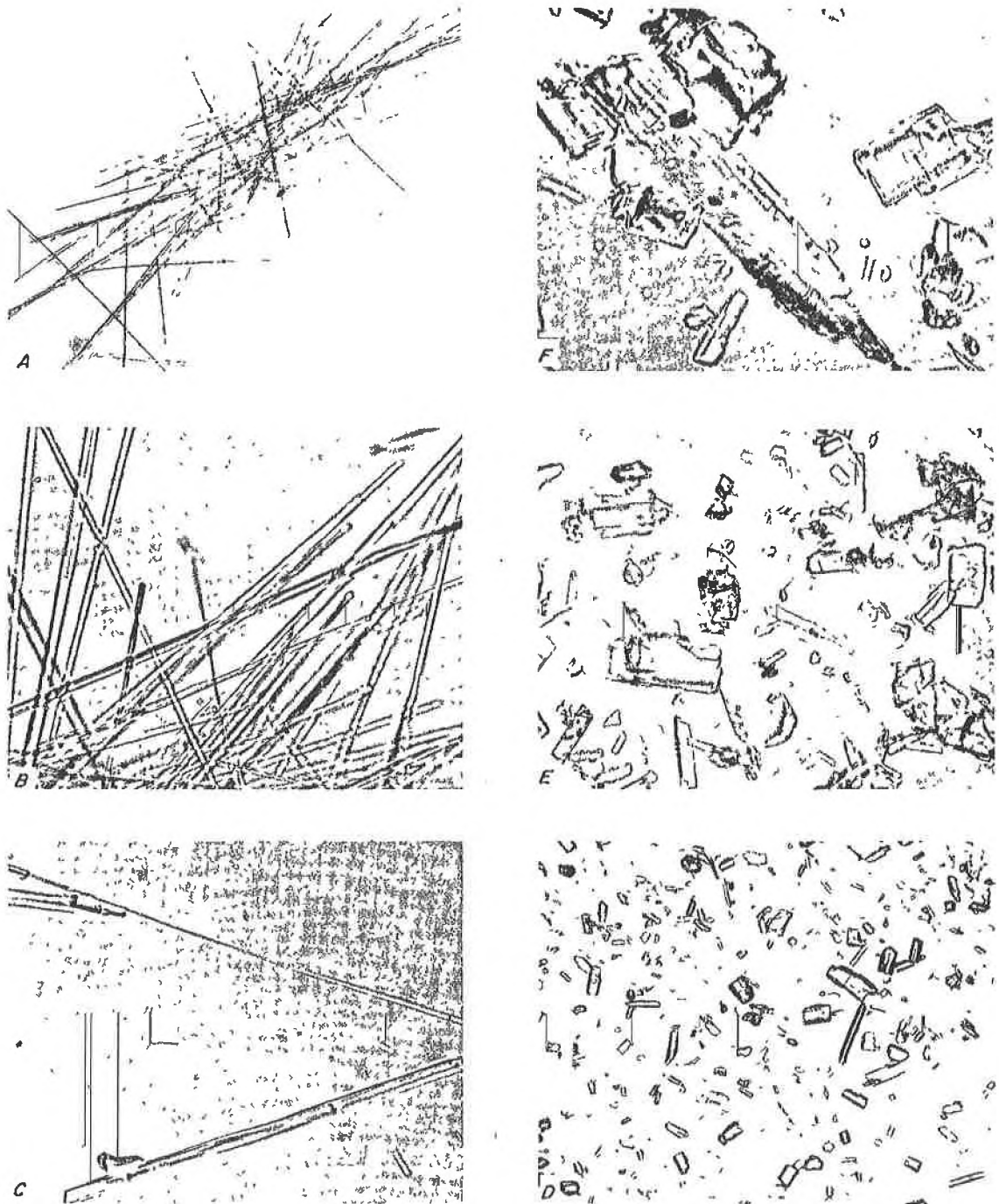
FIGURE 39. • Light optical photomicrographs of tremolite asbestos and tremolite at three magnifications. Tremolite asbestos (left) at A , X 100; B , X 500; and C , X 950. Tremolite (right) at D , X 100; E , X 500; and F , X 950.
