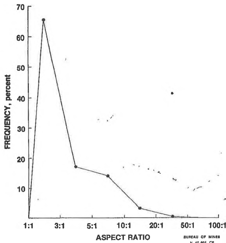
FIGURE 43. - Frequency polygons for the aspect ratio of hornblende.
