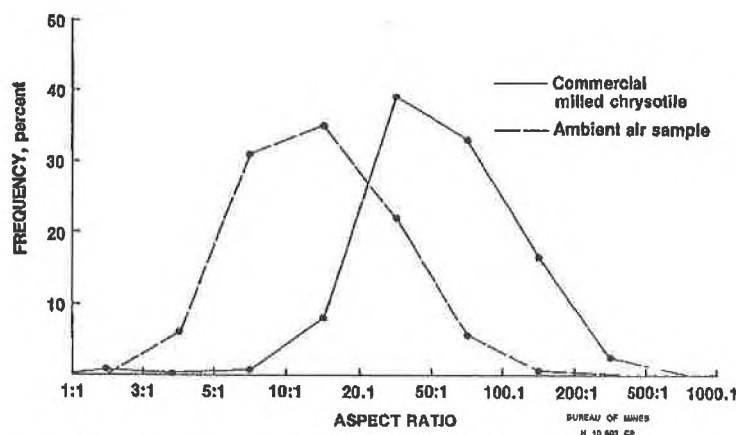
FIGURE 44. - Frequency polygons for the aspect ratios of commercial-grade chrysotile and chrysotile in ambient air.
