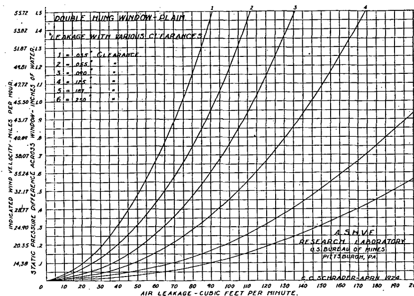
FIG. 6. LEAKAGE THROUGH PLAIN WINDOW WITH VARIOUS CLEARANCES
