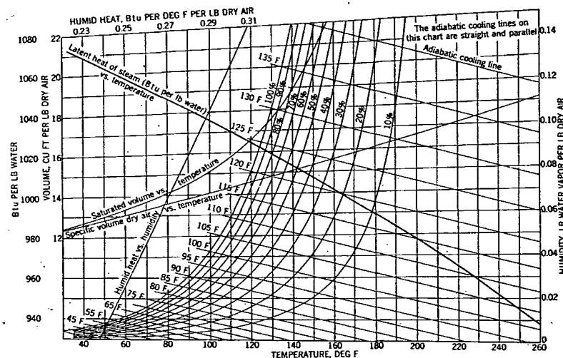
FIG. 6. PSYCHROMETRIC CHART
