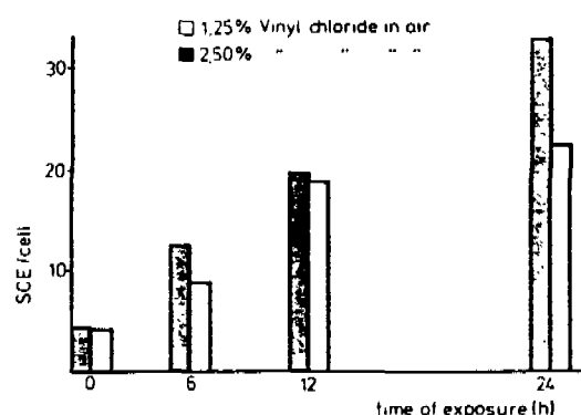
Fig. 2. In vivo induced sister chromatid exchanges in bone marrow chromosomes of Chinese hamster
