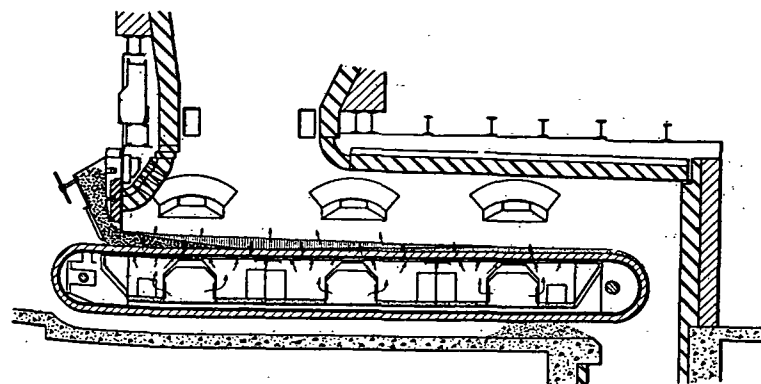
FIG. 8. OVERFEED TRAVELING-GRATE STOKER
