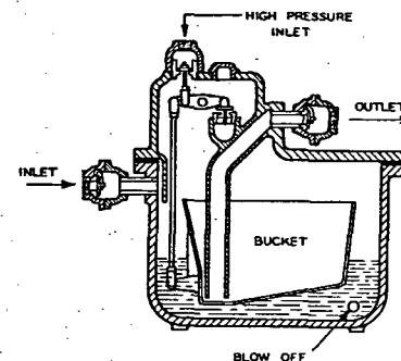
FIG. 32. LIFTING TRAP
