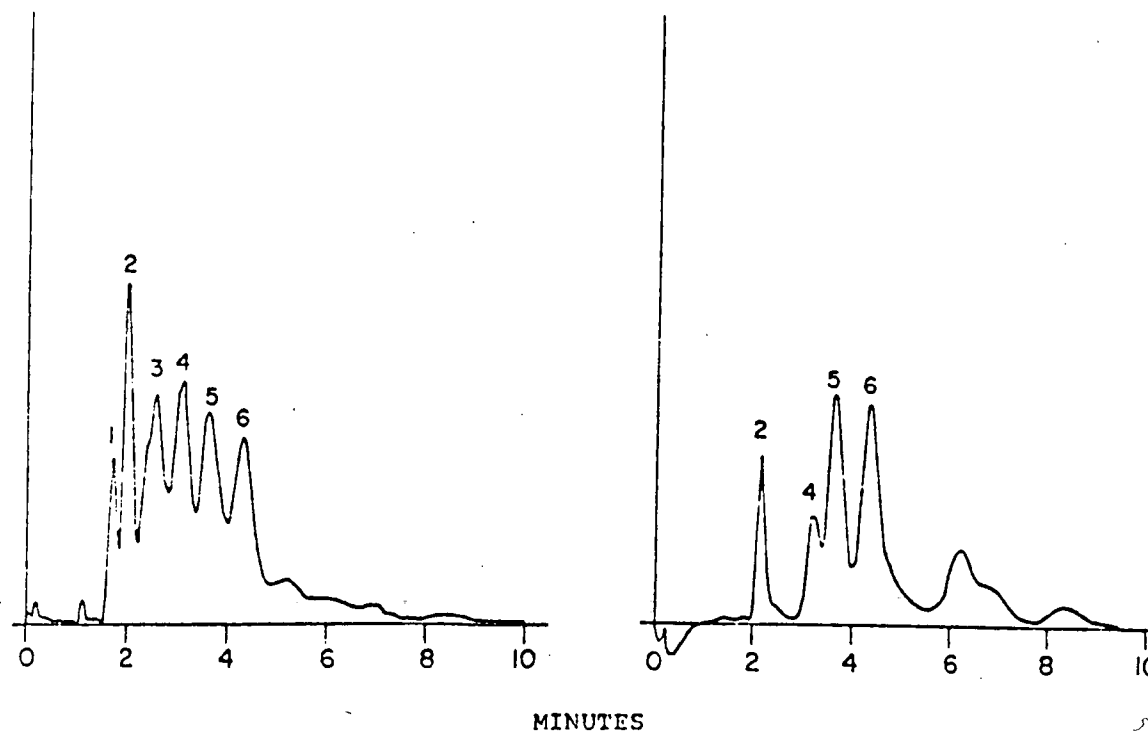
Figure 1 GLC-EC tracings from 24 ng of Aroclor 1254 (left) and from the residue found in the liver of a group 2 rat.
