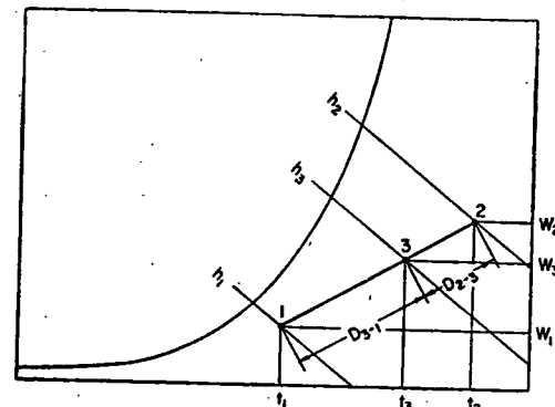
FIG. 11. SOLUTION OF EXAMPLE 5 ON ASHAE PSYCHROMETRIC CHART
