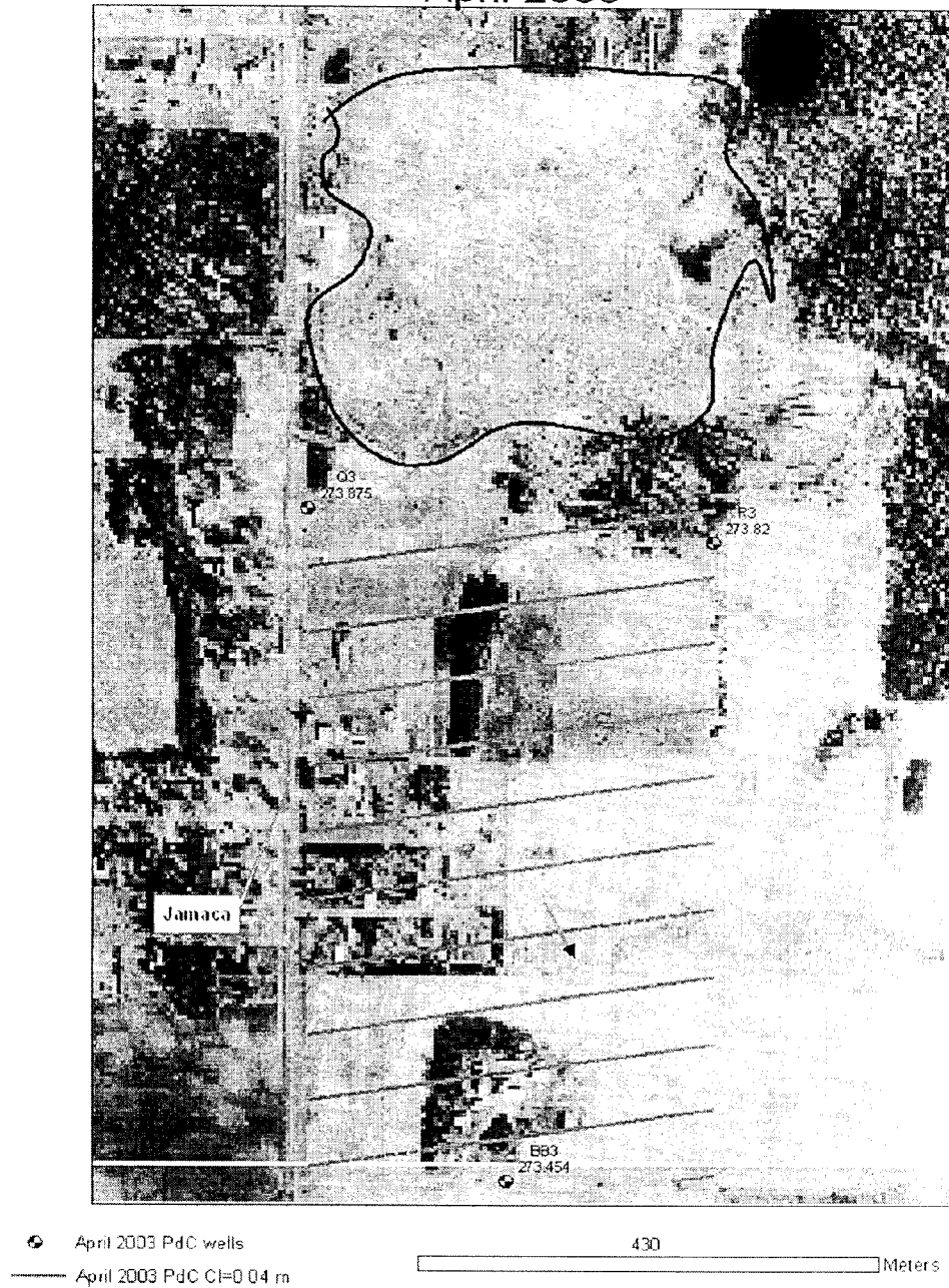
Figure 9 Flow in the Prairie du Chien aquifer April 2003
