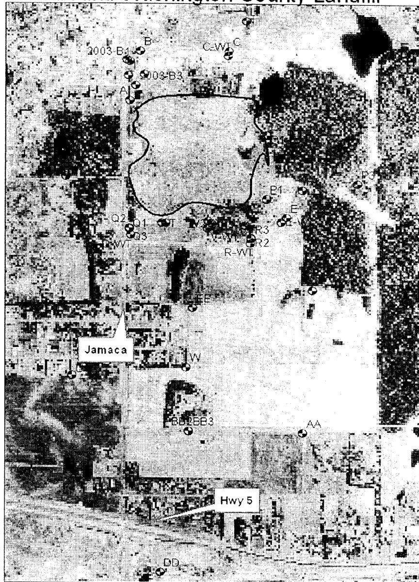
Figure 2 Groundwater Monitoring Network around Washington County Landfill
