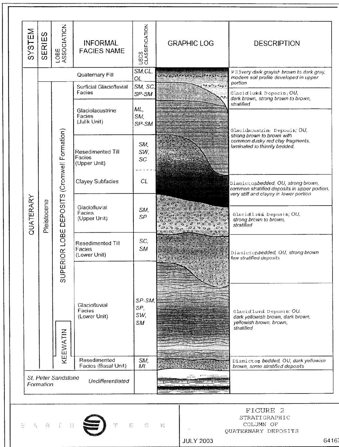
Figure 24 Stratigraphic Column of Quaternary Deposits (Figure 2 from Hydrogeologic Site Characterization Near Well "I" )
