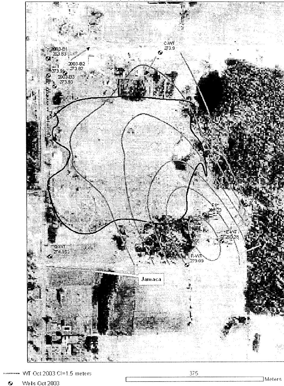
Figure 5 Flow at the water table October 2003
