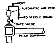
Fig. 12. . . . Typical Automatic Air Vent Valve Installation
