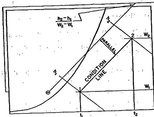
FIG. 16. SOLUTION OF EXAMPLE 8 ON A.S.H.A.E. PSYCHROMETRIC CHART
