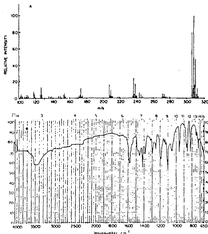
FIG. 3. Mass spectrum (A) and IR spectrum (B) of Metabolite II. The compound was identified as 3-OH-2,5,2',5'-tetrachlorobiphenyl.
