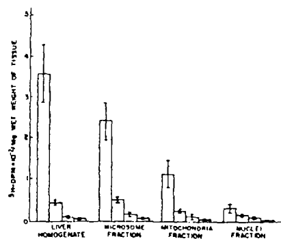
FIG. 2. Distribution of 3 H in liver homogenates and subcellular fractions of liver 1, 3, 7, and 14 days (L to R) following a single oral dose of 3 H-2,5,2',5'-tetrachlorobiphenyl. 1 signifies mean ± 1 SD.
