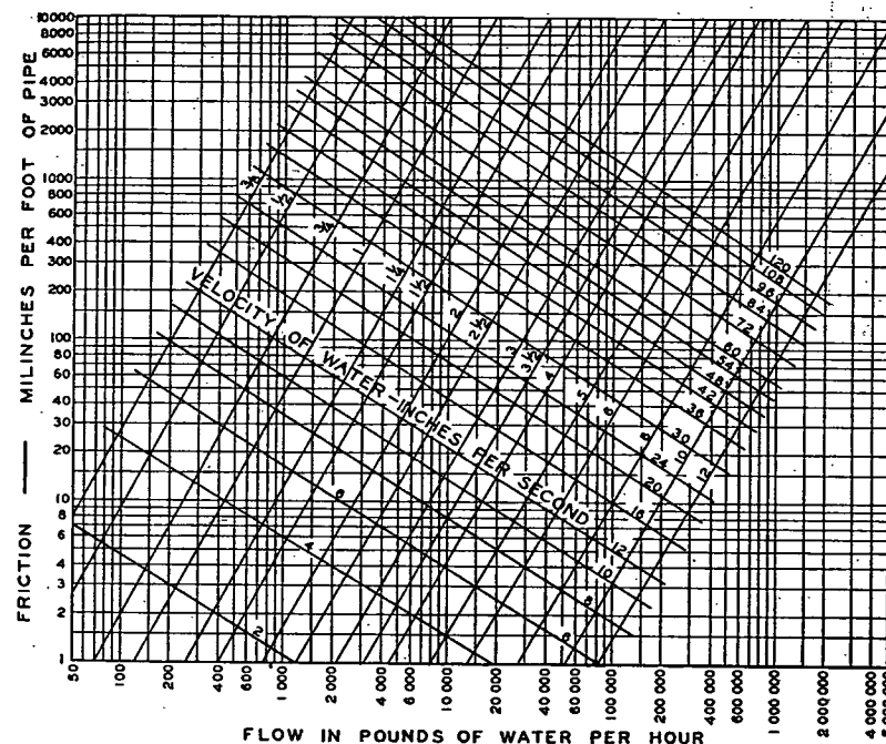
FIG. 2. FRICTION IN BLACK IRON PIPES BASED ON FLOW IN POUNDS PER HOUR
