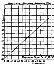
DENSITY OF MONOSODIUM PHOSPHATE SOLUTIONS
