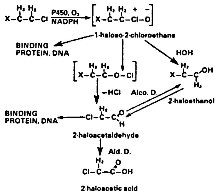
Figure 9-5 Microsomal oxidative metabolism of 1,2-dihaloethanes. Source: Adapted from Guengerich et al. (1980), Anders and Livesey (1980).
