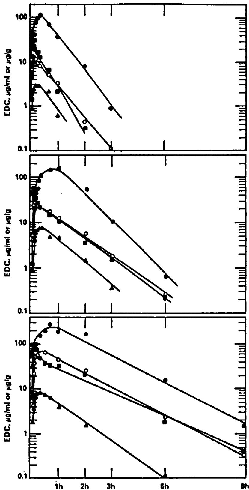
Figure 9-1 EDC levels after single oral administration in rats: Top panel, 25 mg/kg; middle, 50 mg/kg; bottom, 150 mg/kg dose. Adipose tissue (●), blood (○), liver (■), lung (▲). Source: Spreafico et al. (1978, 1979, 1980).
