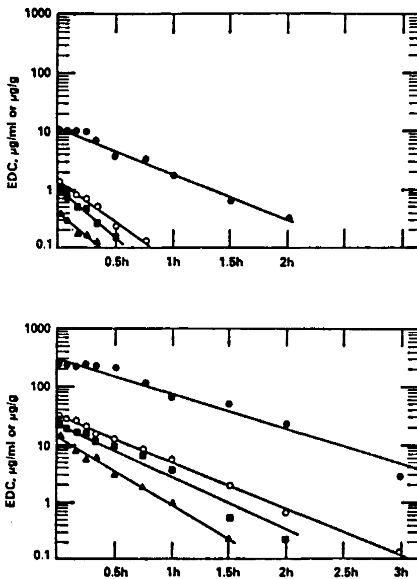
Figure 9-4 Levels of EDC in rats after inhalatory exposure to 50 ppm (top) and 250 ppm (bottom). Levels were measured at termination of 5-hour exposure period. Adipose tissue (●), blood (○), liver (■), lung (▲). Source: Spreafico et al. (1978, 1979, 1980).
