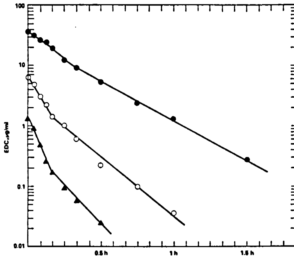
Figure 9-3 Blood levels of EDC in rats after i.v. administration. (●) 25 mg/kg i.v.; (○) 5 mg/kg i.v.; (▲) 1 mg/kg i.v. Source: Spreafico et al. (1978, 1979, 1980).
