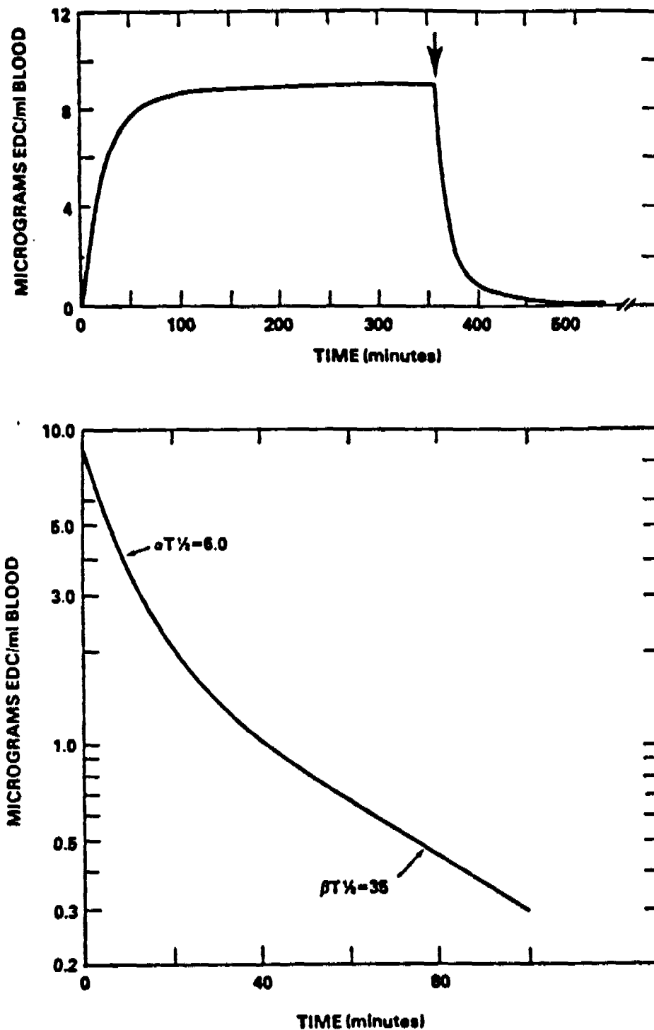
Figure 9-2 Top: Blood levels of EDC observed during and following a 6-hour inhalation exposure to 150 ppm EDC. Data from four male Osborne-Mendel rats were fitted to a two-compartment open model as described by Gehring et al. 35 The computer plot is shown. The arrow indicates exposure termination. Bottom: Semi-logarithmic plot of EDC blood levels vs. time after exposure termination. Source: Reitz et al. (1980, 1982).
