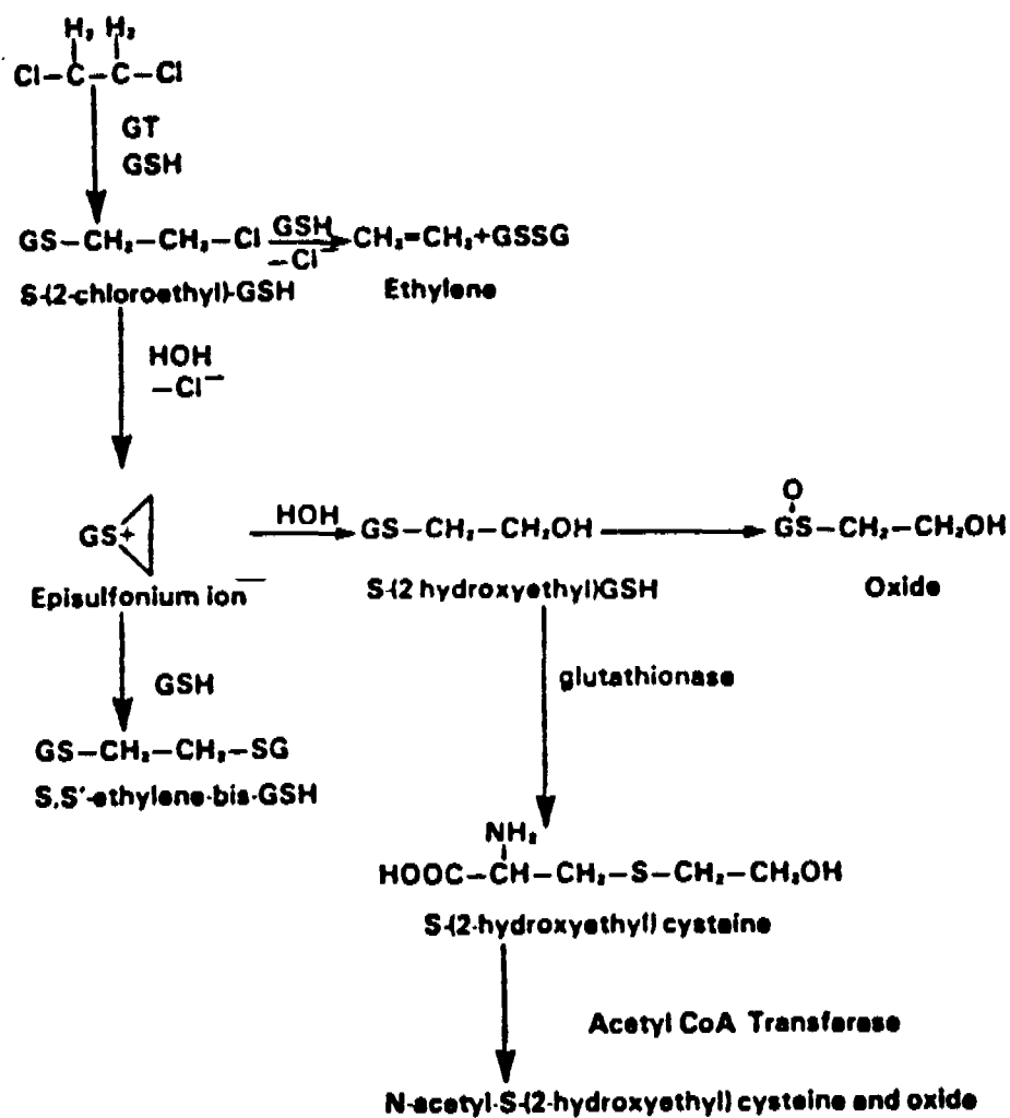
Figure 9-7 . Cytosolic metabolism of ethylene dichloride. Source: Adapted from Anders and Livesey (1980).
