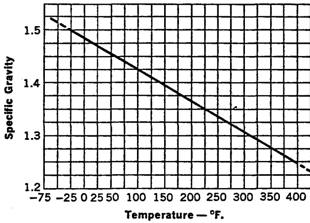
THERMINOL® FR Lo-Temp Specific Gravity
