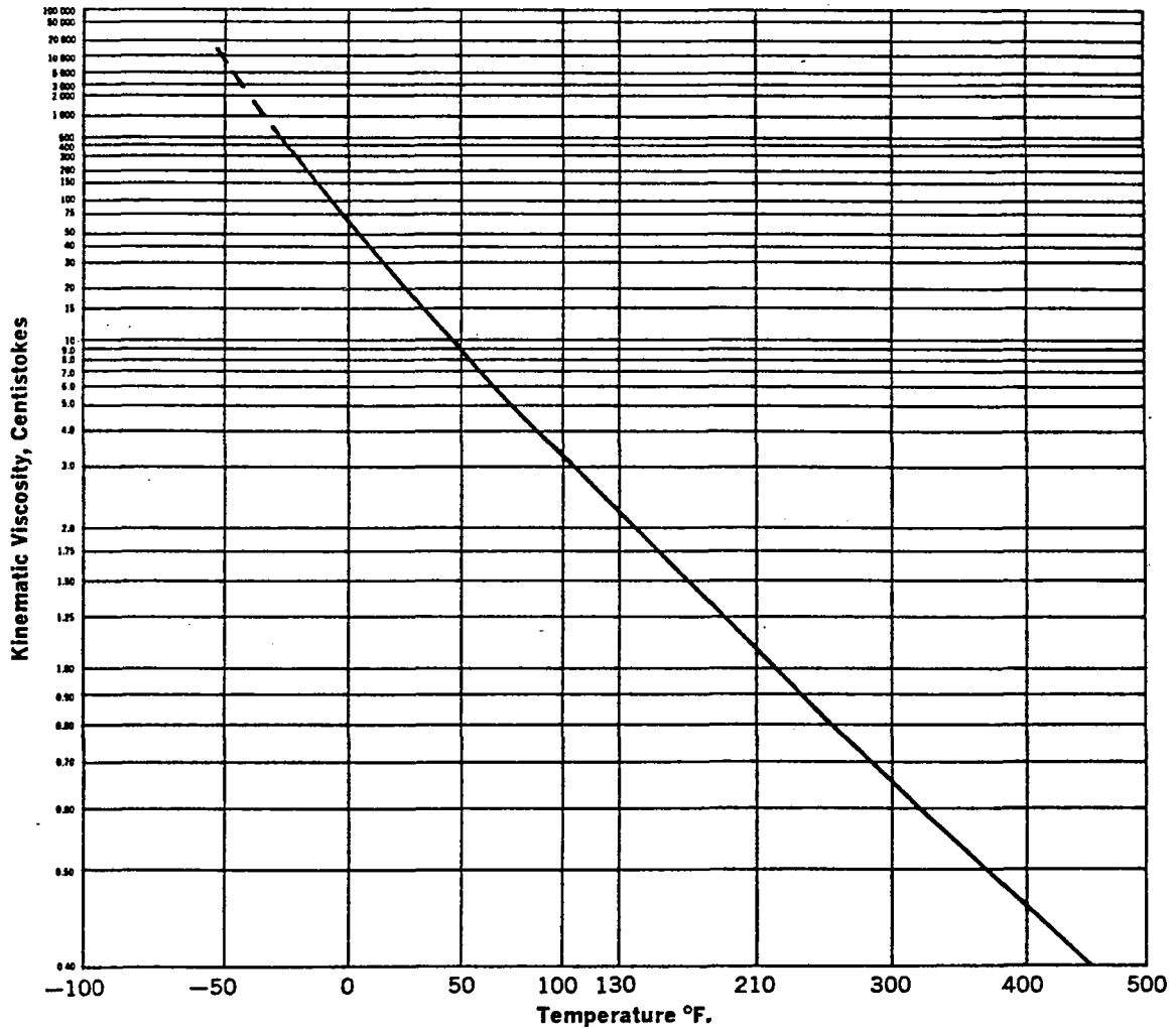
THERMINOL® FR Lo-Temp Viscosity
