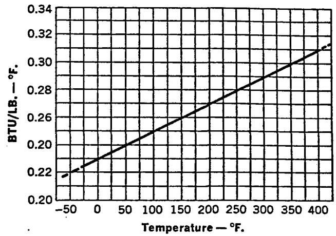
THERMINOL® FR Lo-Temp Specific Heat
