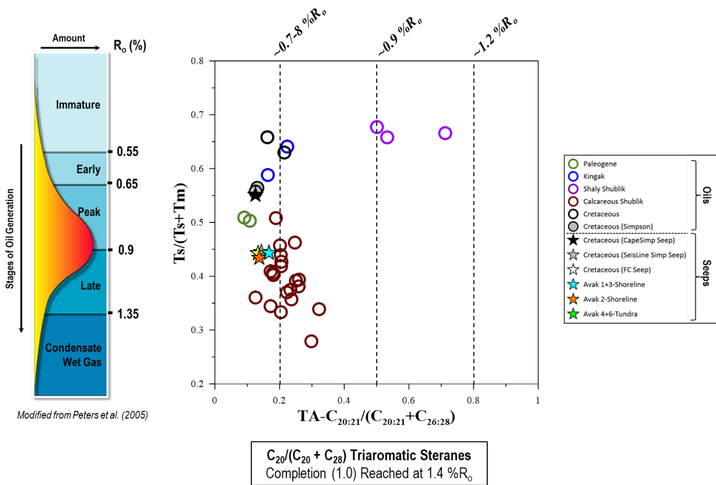
Figure 11. Thermal Maturity. Increasing values of TA-(C_{20:21})/(C_{20:21}+C_{26:28}) relative to Ts/(Ts+Tm) reflect a general increase in thermal maturation as indicated by dashed lines and estimated vitrinite reflectance values at top according to the TA - R_o relationship defined in Peters et al. (2005).
