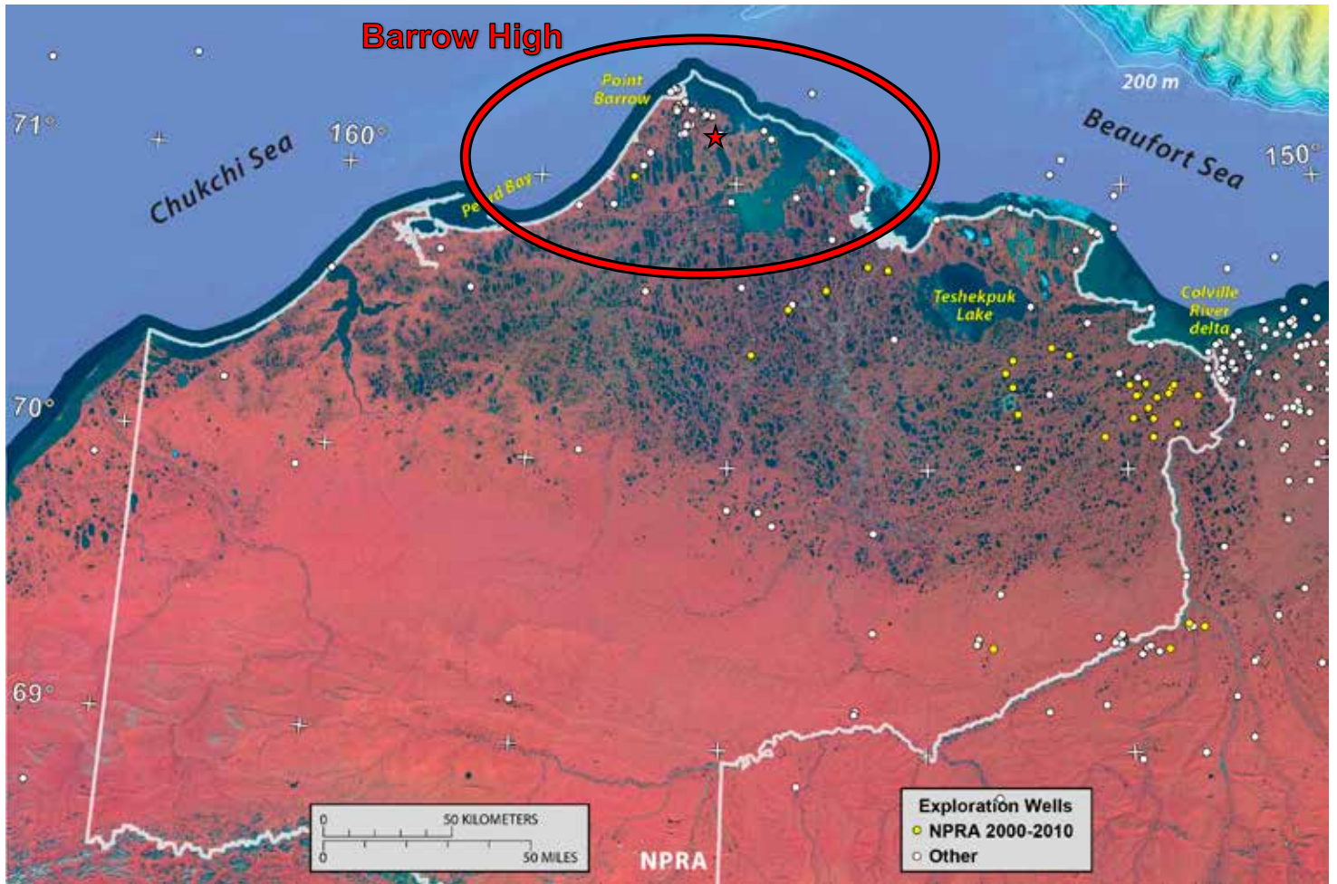
Figure 3. False-color composite Landsat image of northernmost Alaska showing in white the boundary of the National Petroleum Reserve in Alaska (NPRA). Petroleum exploration wells drilled prior to 2000 are shown as white dots and those drilled during 2000 to 2010 are shown as yellow dots. Red oval outlines the “Barrow High,” an area of high-standing basement rocks in the subsurface. Red star shows location of Avak Creek oil occurrence.
