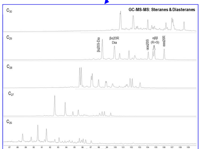
Figure 10. Analytical Chromatograms: GC-FID (whole oil) → GC-MS (saturate fraction) → GC-MS-MS (saturate fraction). Advanced instrumentation allowed for removal of overlapping hydrocarbons and peak interferences to provide a more accurate view of hydrocarbon profiles and identification of hydrocarbon peaks.
