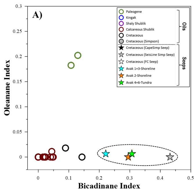
Figure 13. Source age and organic matter. Age-diagnostic (and taxon-specific) biomarker parameters used to bracket age ranges and discriminate oil families. A) Bicadinane and oleanane indices are highly specific for both Cretaceous and younger sources and terrestrial plant organic matter input. B) Sterane distributions discriminate source organic matter contributions (e.g., marine algal flora, diatoms, terrigenous plant input). Abbreviations: oleanane index ( ((\alpha\text{-oleanane} + \beta\text{-oleanane})/(\alpha\text{-oleanane} + \beta\text{-oleanane} + \text{C}_{30}\text{H})) ); bicadinane index ( (\text{bicadinane-T}/(\text{bicadinane-T} + \text{C}_{30}\text{H})) ).
