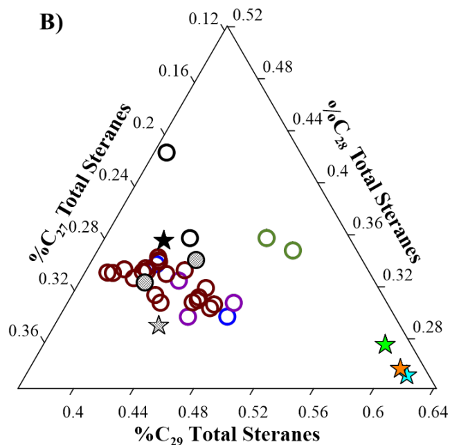
Figure 13. Source age and organic matter. Age-diagnostic (and taxon-specific) biomarker parameters used to bracket age ranges and discriminate oil families. A) Bicadinane and oleanane indices are highly specific for both Cretaceous and younger sources and terrestrial plant organic matter input. B) Sterane distributions discriminate source organic matter contributions (e.g., marine algal flora, diatoms, terrigenous plant input). Abbreviations: oleanane index ( ((\alpha\text{-oleanane} + \beta\text{-oleanane})/(\alpha\text{-oleanane} + \beta\text{-oleanane} + \text{C}_{30}\text{H})) ); bicadinane index ( (\text{bicadinane-T}/(\text{bicadinane-T} + \text{C}_{30}\text{H})) ).
