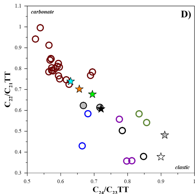
Figure 12. Lithology-sensitive bulk geochemical (A, B) and biomarker parameters (C, D). Among samples of similar thermal maturity, variation in source-related parameters represent differences in lithofacies of the inferred generating source rock among oil families (Seifert and Moldowan, 1978; Sieskind et al., 1979; Zumberge, 1984; Moldowan et al., 1986, 1991; Peters et al., 2005). Stable carbon isotopes of C_{15+} saturate and aromatic hydrocarbon fractions used to discriminate oil samples generated from a predominance of marine or terrestrial source organic matter as defined by Sofer (1984).
