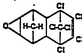
DIELDRIN
