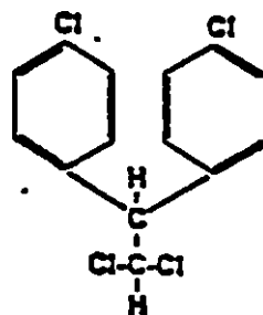
DDD
