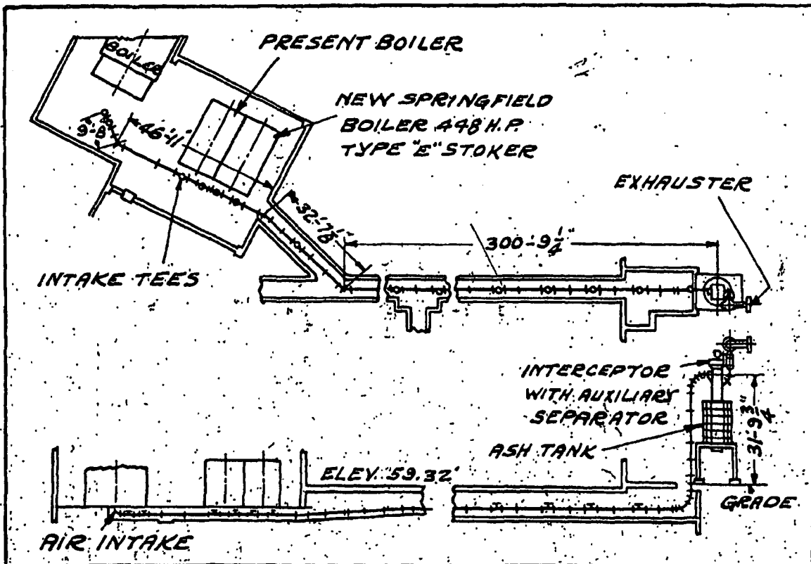
FIG. 1.—Diagrammatic layout showing location of building, conveyor and pipe line, and "Pneumatron" system. Richmond Brothers Co., Cleveland, Ohio.
