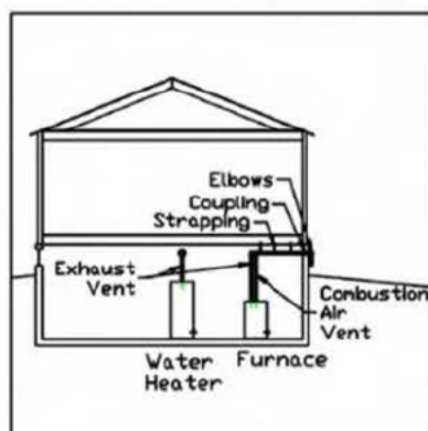
Figure 8D.3.3 Plastic PVC Installation (Condensing Example)
