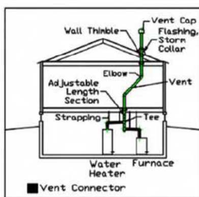
Figure 8D.3.2 Metal Venting Installation (Non-Condensing Gas-fired Water Heater and/or Non-Condensing Gas-fired Furnace)
