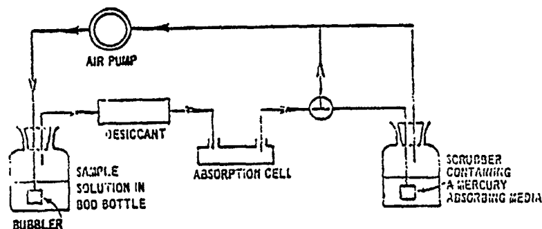
Figure 105-1. Apparatus for flameless mercury determination.
