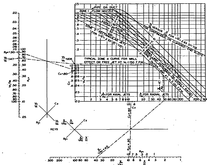
Fig. 2. ... Chart for Determining Centerline Velocities of Axial and Radial Jets
