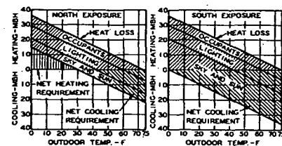
Scale: Floor area—1000 sq ft. Windows on one side only—240 sq ft. Heat transmission factors, U, roof—0.15, wall—0.25, glass—1.13. No infiltration. Heat gain based on artificial lighting at 2.5 watts per sq ft of floor area. Occupants, 35. Solar intensity and incidence at 45 deg N. latitude, December 1. Windows shaded by venetian blinds. Since the consideration is cooling, a room temperature of 75 F, instead of the 72 F shown in Table 1, was used in the above charts. Net cooling requirement for the south exposure approaches that of the north exposure on a day when the sky has a heavy cloud cover.
