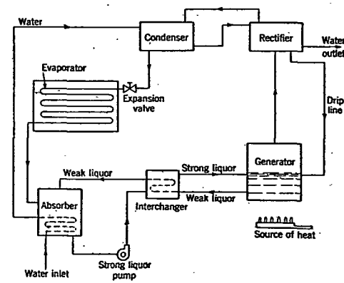
FIG. 6. CLOSED ABSORPTION SYSTEM
