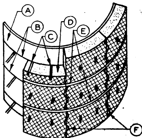
FIGURE 10. Blanket insulation held on by tie wires attached to wire girdles and exterior circumferential bands.
