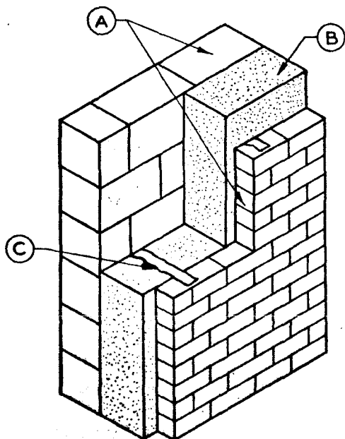
FIGURE 2. Insulation enclosed between masonry walls. A, Masonry walls; B, mineral wool insulation; C, metal tie.
