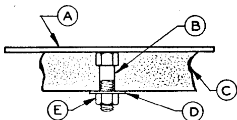
FIGURE 6. Insulation attached by bolts with heads welded to metal surface. A, Heated surface; B, bolt; C, mineral wool insulation; D, washer; E, nut.
