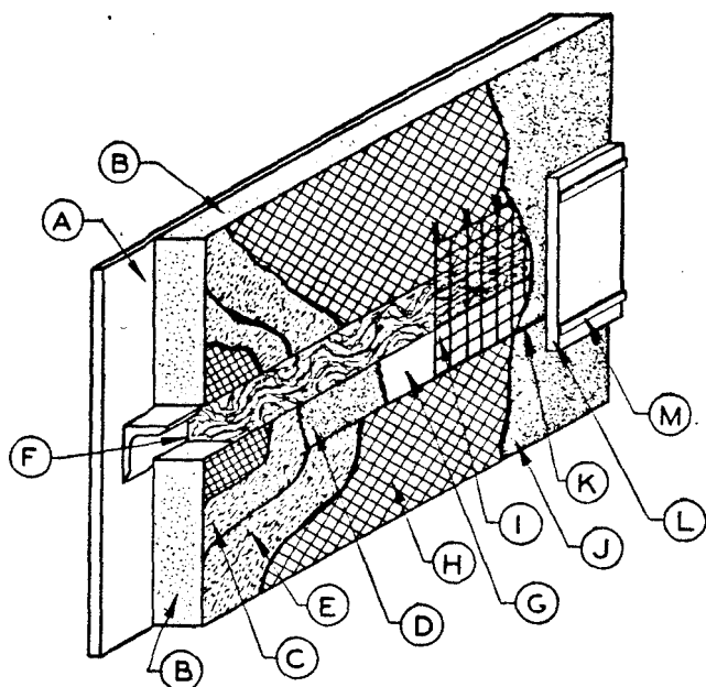
FIGURE 12. Expansion joints for large metal vessels (see par. 16d).
