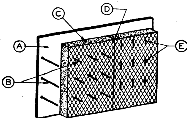
FIGURE 4. Blanket insulation impaled on wires.
