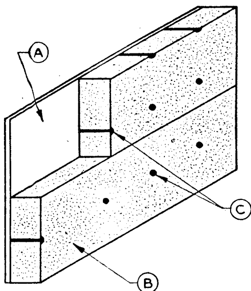
FIGURE 5. Insulation attached by welding with stud gun after insulation is in place. A, Heated surface; B, mineral wool insulation; C, large head studs.
