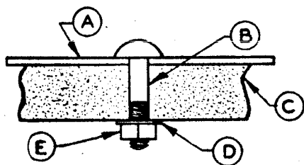
FIGURE 7. Insulation attached by bolts through drilled holes. A, Heated surface; B, bolt; C, mineral wool insulation; D, washer; E, nut.
