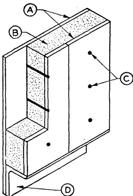
FIGURE 1. Insulation enclosed between metal sheets. A, Metal sheets; B, mineral wool insulation; C, fastenings; D, horizontal support.
