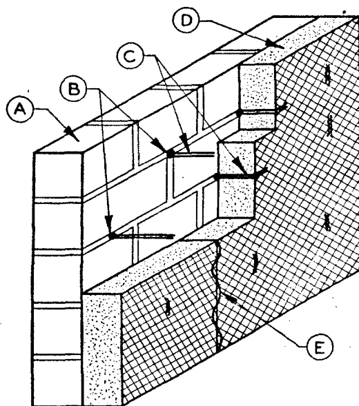
FIGURE 11. Application of blanket insulation by hairpin wires affixed to nails embedded in masonry joints.
