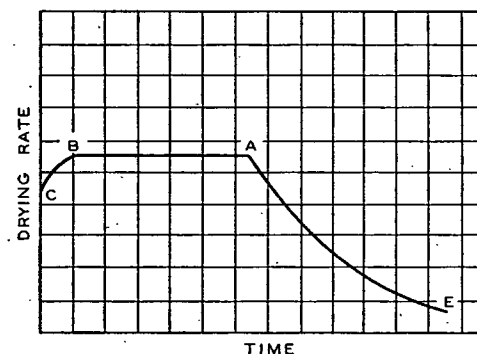
FIG. 4. RATE OF DRYING, \frac{dW}{d\theta} vs. TIME \theta
