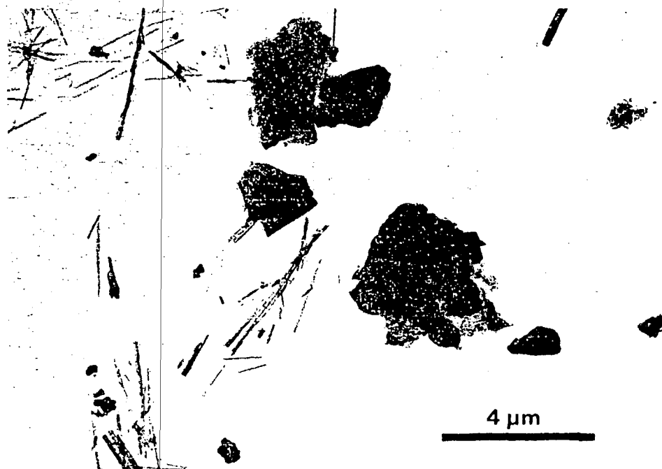
FIG. 5. Chrysotile fibers associated with talc particles.
