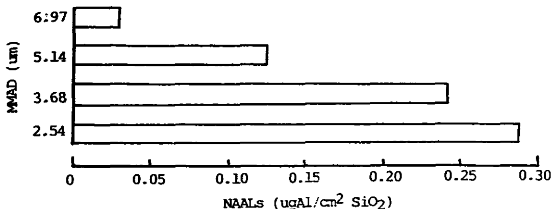
Figure 3. The net amounts of Al (NAALs) combined on the SiO 2 particles of various diameter (MMAD 2.54 to 6.97μm) sampled by cascade impactor (10L/min sampling flow rate).
