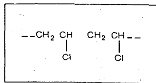
Fig 2.—Polyvinyl chloride.
