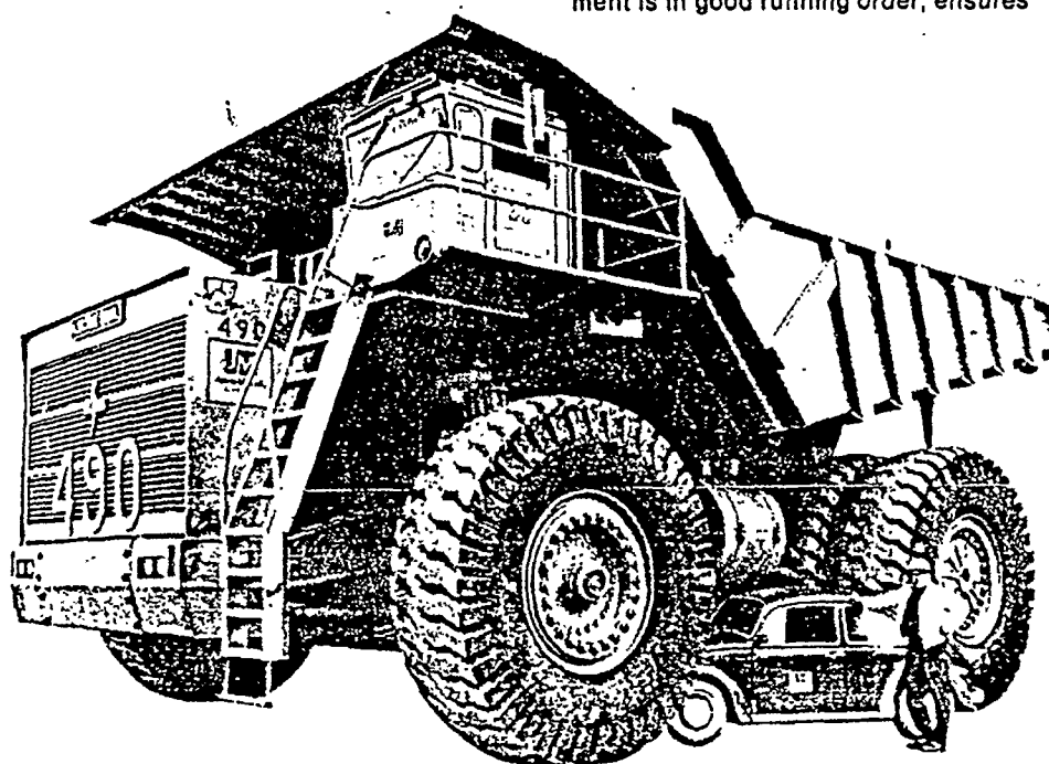
At left, gigantic 200-ton truck dwarfs man. At right, a special vehicle equipped with a boom has been designed in the mines to change loaded truck tires without causing damage.
