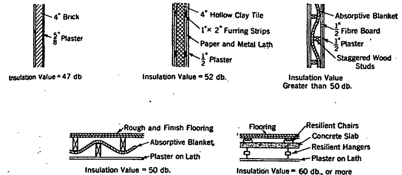
FIG. 1. THREE WALL SECTIONS AND TWO FLOOR AND CEILING SECTIONS WHICH ARE SUITABLE FOR THE INSULATION OF EQUIPMENT ROOMS a
