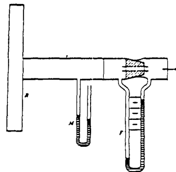
FIG. 1 ARRANGEMENT FOR TESTING THE RESISTANCE TO AIR FLOW OF VARIOUS FORMS OF RESPIRATORS (R = respirator, M = water manometer, F = flow meter with capacity of 85 liters per minute.)
