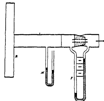
FIG. 1 ARRANGEMENT FOR TESTING THE RESISTANCE TO AIR FLOW OF VARIOUS FORMS OF RESPIRATORS (R = respirator, M = water manometer, F = flow meter with capacity of 85 liters per minute.)
