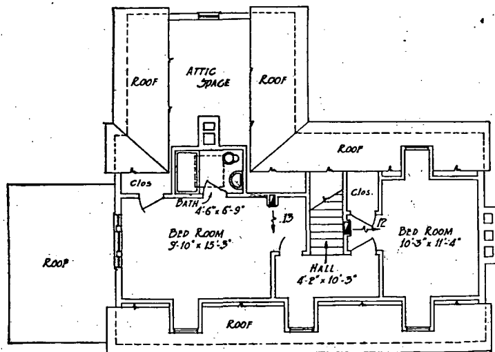
FIG. 11. THIRD-FLOOR PLAN, RESEARCH RESIDENCE
