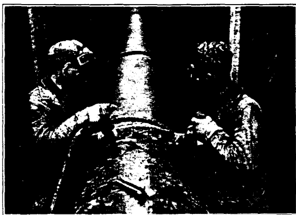
COURTESY U. S. PIPE & FOUNDRY CO. Calking poured lead joints with pneumatic hammers
