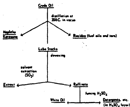
Outline of a petroleum fractionation.
