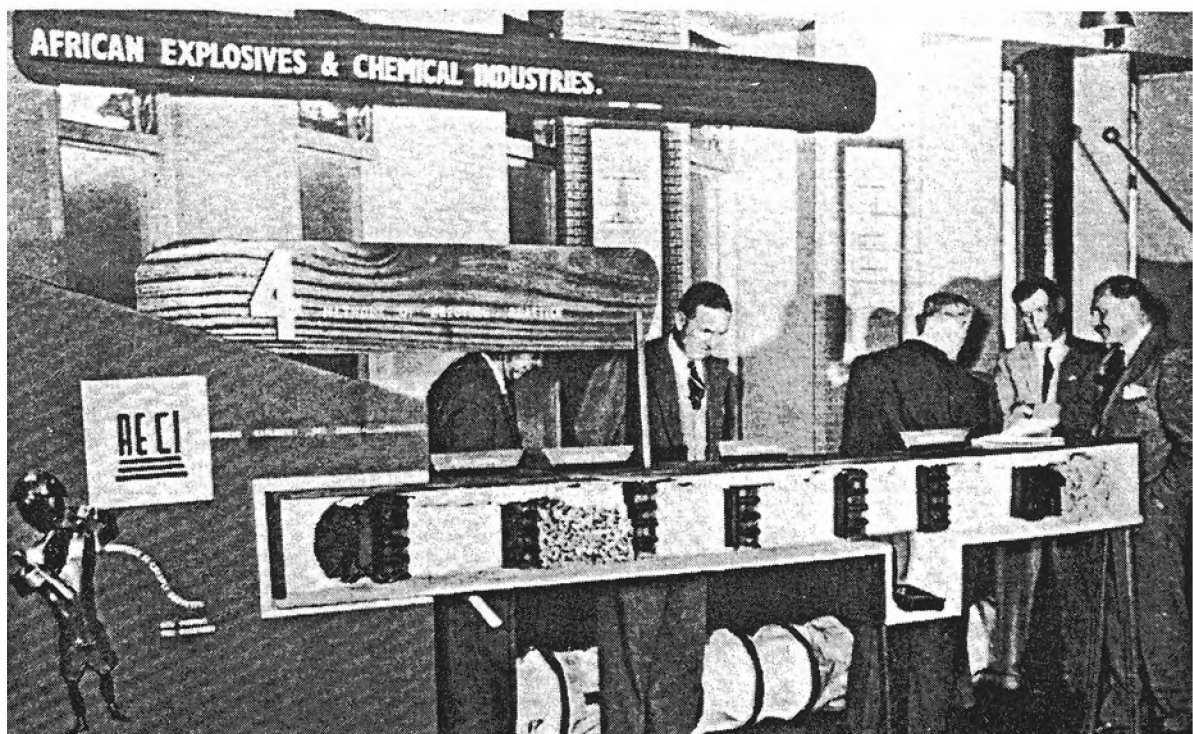
The model of a stope exhibited by African Explosives and Chemical Industries, showing four different methods of erecting "Vynide" brattice cloth for controlling air-flow.
