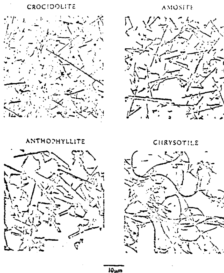
Fig. 6. [From Timbrell, V.: Physical factors as etiologic mechanisms, in Biological Effects of Asbestos , IARC Scientific Publication No. 8, Lyon, 1973, p. 233; reprinted by permission of publisher.] Electron micrographs of crocidolite (north western Cape Province), amosite (Transvaal), anthophyllite (Finland), chrysotile (Canada) at the same magnification ( \times 1700 ). Features to note are (1) the rectilinear shape of the amphibole fibers compared with the curved and beaded morphology of chrysotile fibers; (2) the order of the diameters of the amphibole fibers, suggested by numerous electron micrographic examinations of these fibers from the 3 geographical areas, crocidolite < amosite < anthophyllite; (3) the longitudinal fragmentation of the chrysotile fibers and the small diameter (about 0.03 \mu\text{m} ) of the ultimate fibrils.
